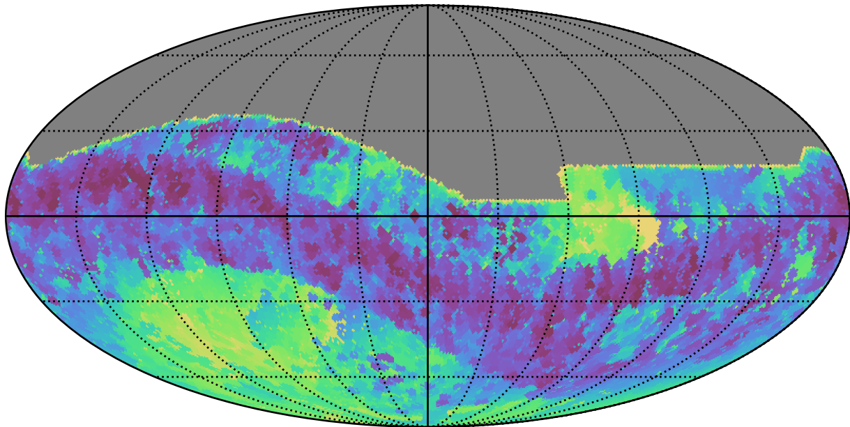
weather_cloudso10v3.4_10yrs All sky i band: Min skyBrightness
