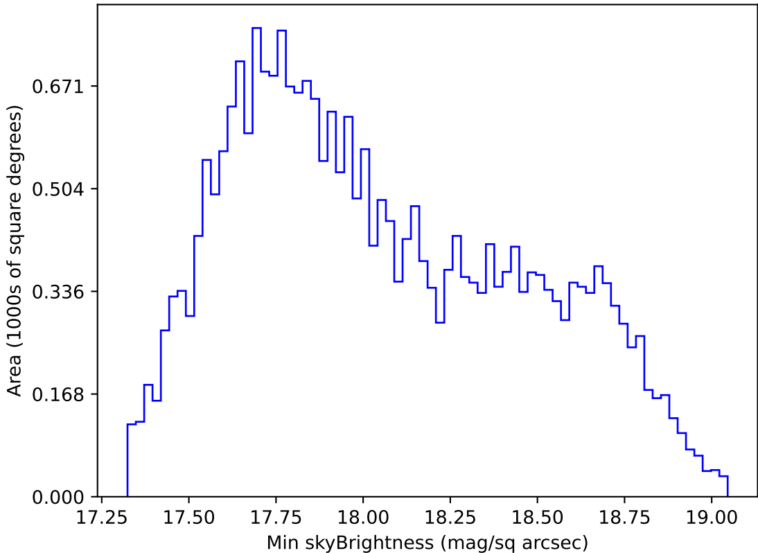
weather_cloudso10v3.4_10yrs All sky i band: Min skyBrightness
