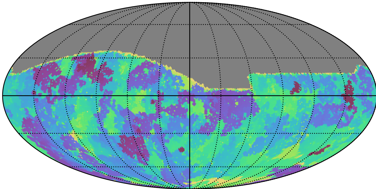
weather_cloudso10v3.4_10yrs All sky g band: Min skyBrightness
