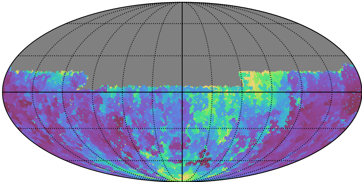
weather_cloudso10v3.4_10yrs Yr 1 u band: Min seeingGeom
