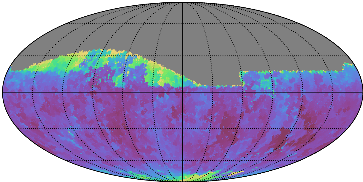
weather_cloudso10v3.4_10yrs Yr 1 r band: Min seeingGeom
