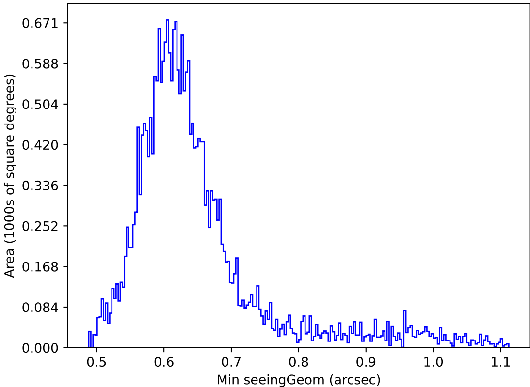
weather_cloudso10v3.4_10yrs Yr 1 r band: Min seeingGeom
