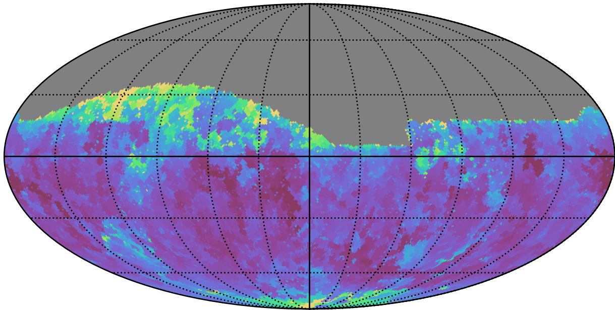
weather_cloudso10v3.4_10yrs Yr 1 z band: Min seeingEff
