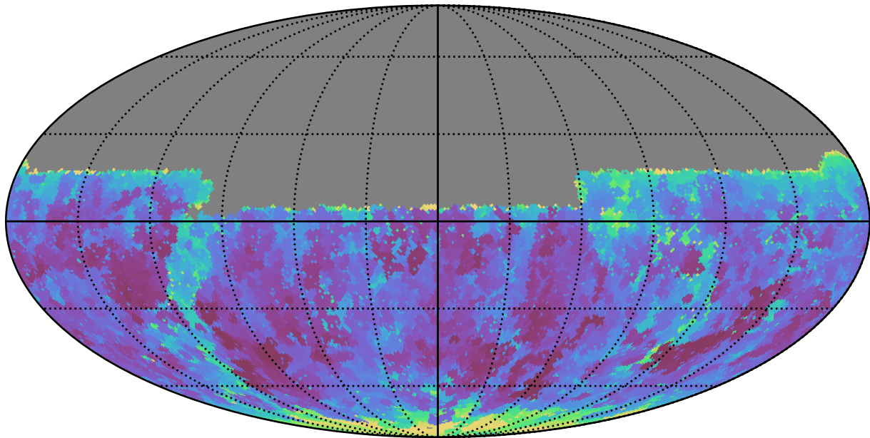
weather_cloudso10v3.4_10yrs Yr 1 y band: Min seeingEff
