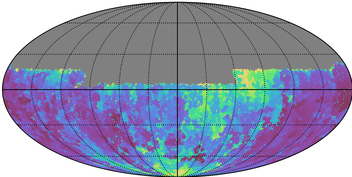
weather_cloudso10v3.4_10yrs Yr 1 u band: Min seeingEff
