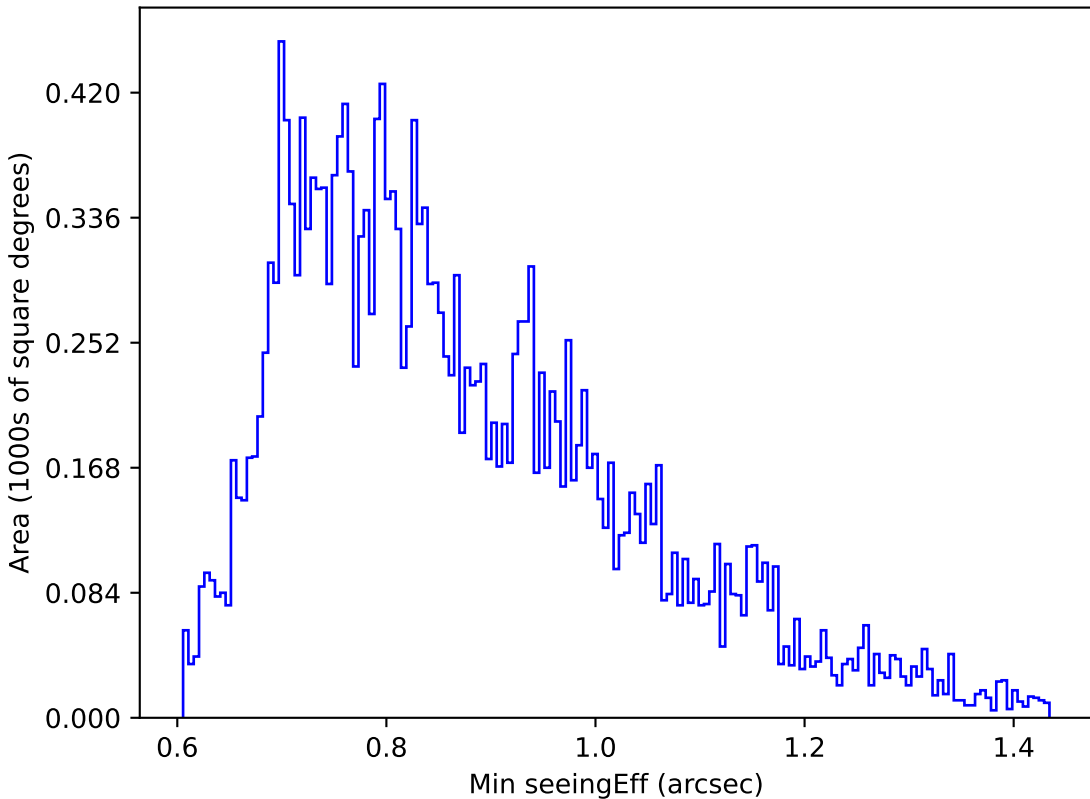
weather_cloudso10v3.4_10yrs Yr 1 u band: Min seeingEff
