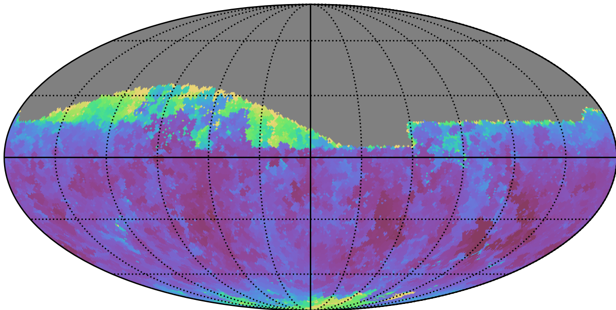
weather_cloudso10v3.4_10yrs Yr 1 r band: Min seeingEff
