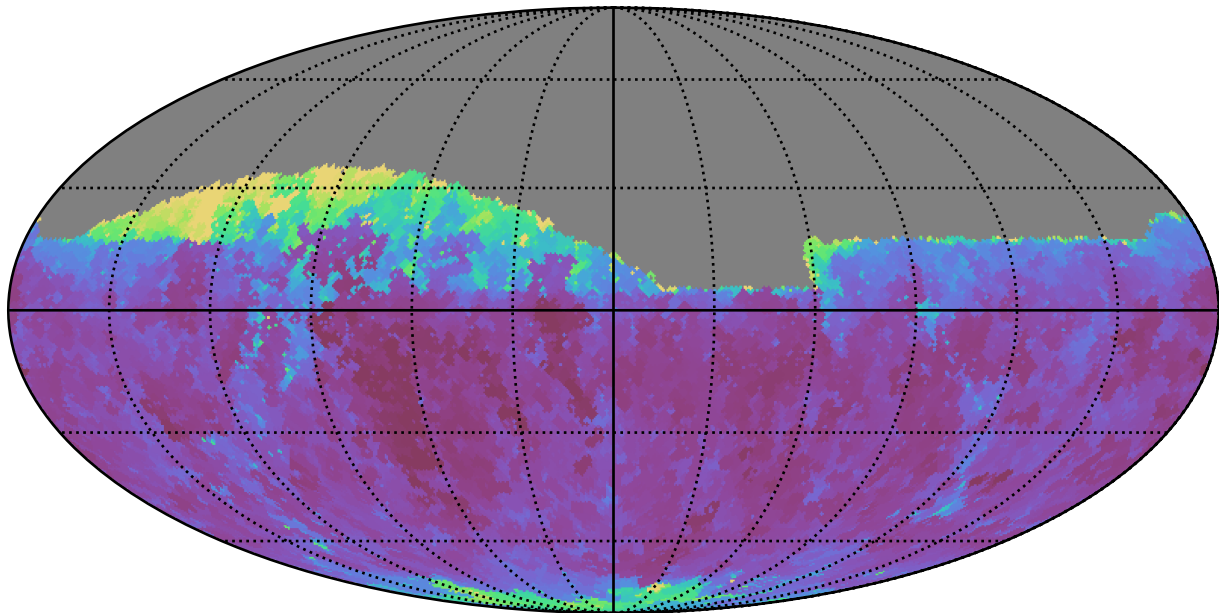
weather_cloudso10v3.4_10yrs Yr 1 i band: Min seeingEff
