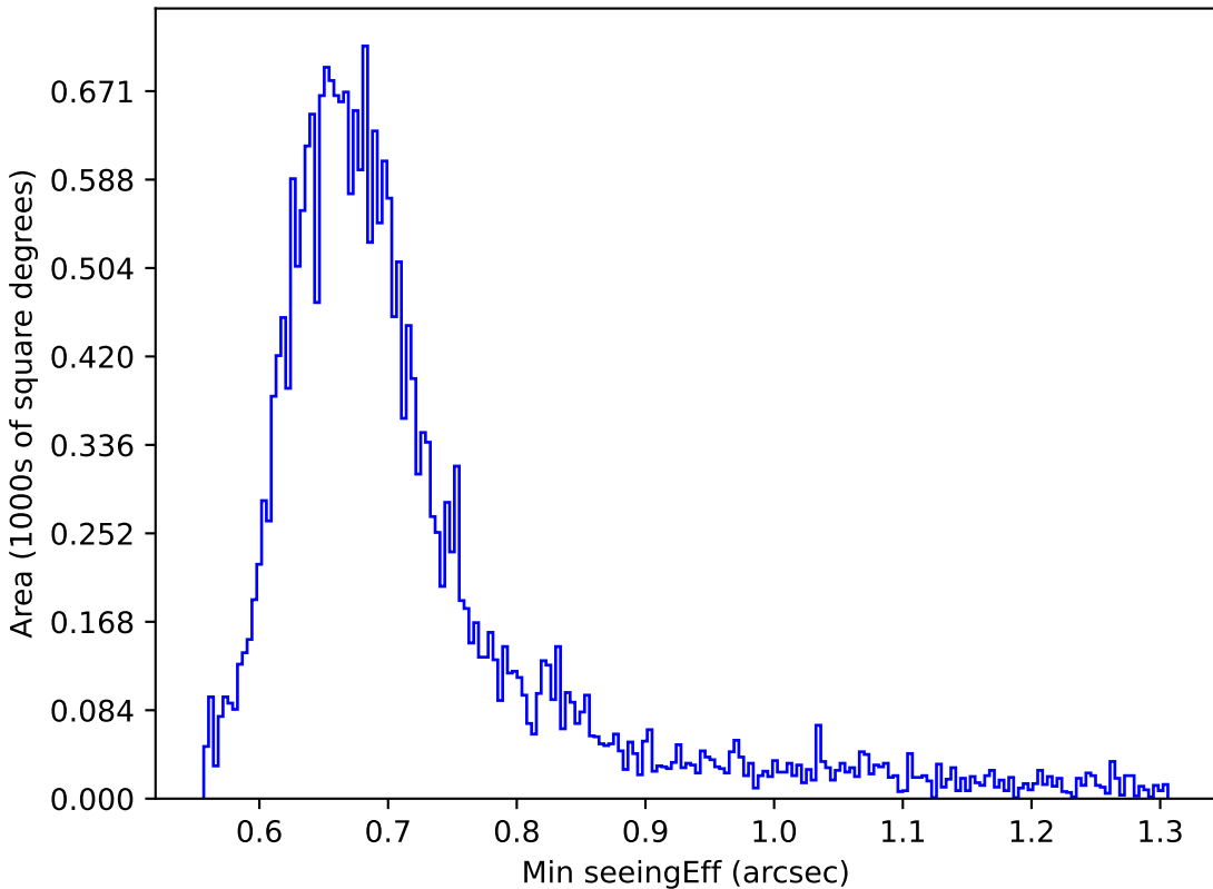
weather_cloudso10v3.4_10yrs Yr 1 i band: Min seeingEff
