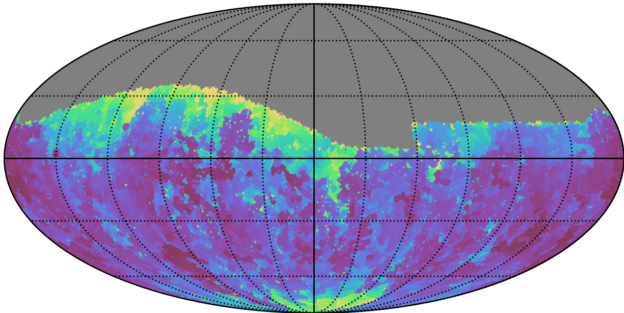
weather_cloudso10v3.4_10yrs Yr 1 g band: Min seeingEff
