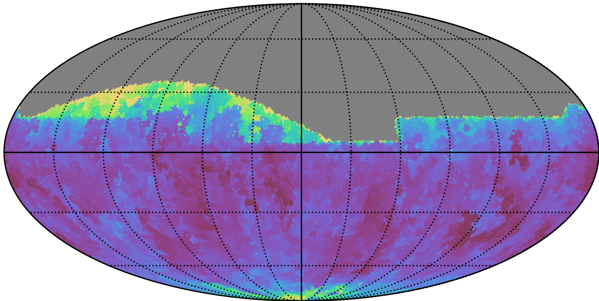
weather_cloudso10v3.4_10yrs Yr 1 all bands: Min seeingEff
