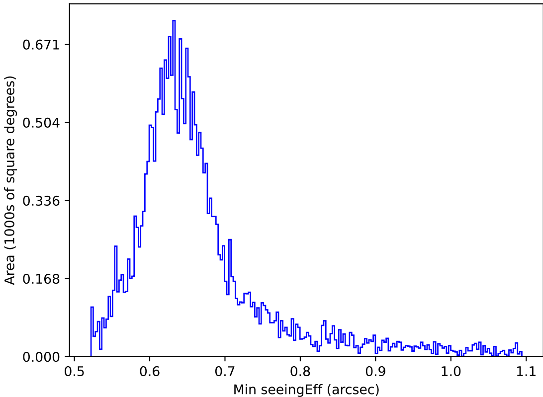
weather_cloudso10v3.4_10yrs Yr 1 all bands: Min seeingEff
