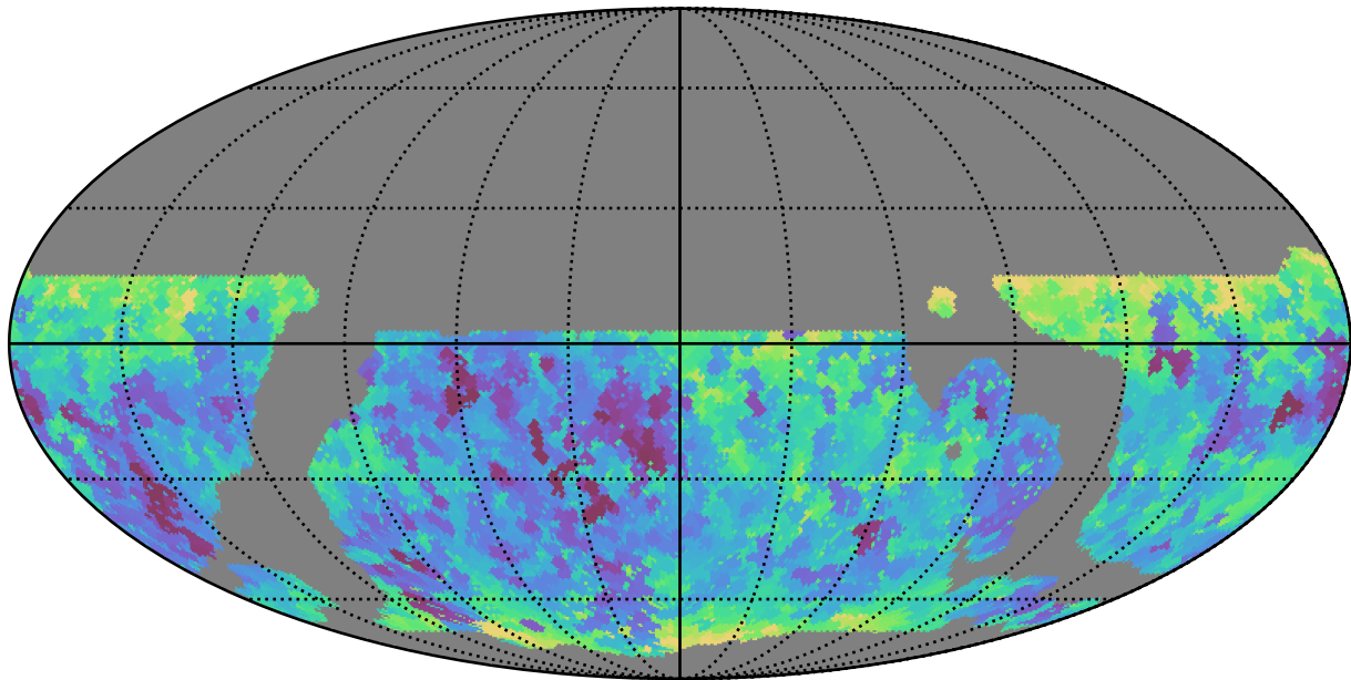
weather_cloudso10v3.4_10yrs WFD z band: Min seeingEff
