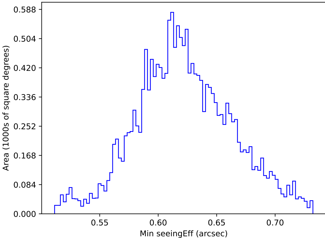
weather_cloudso10v3.4_10yrs WFD z band: Min seeingEff
