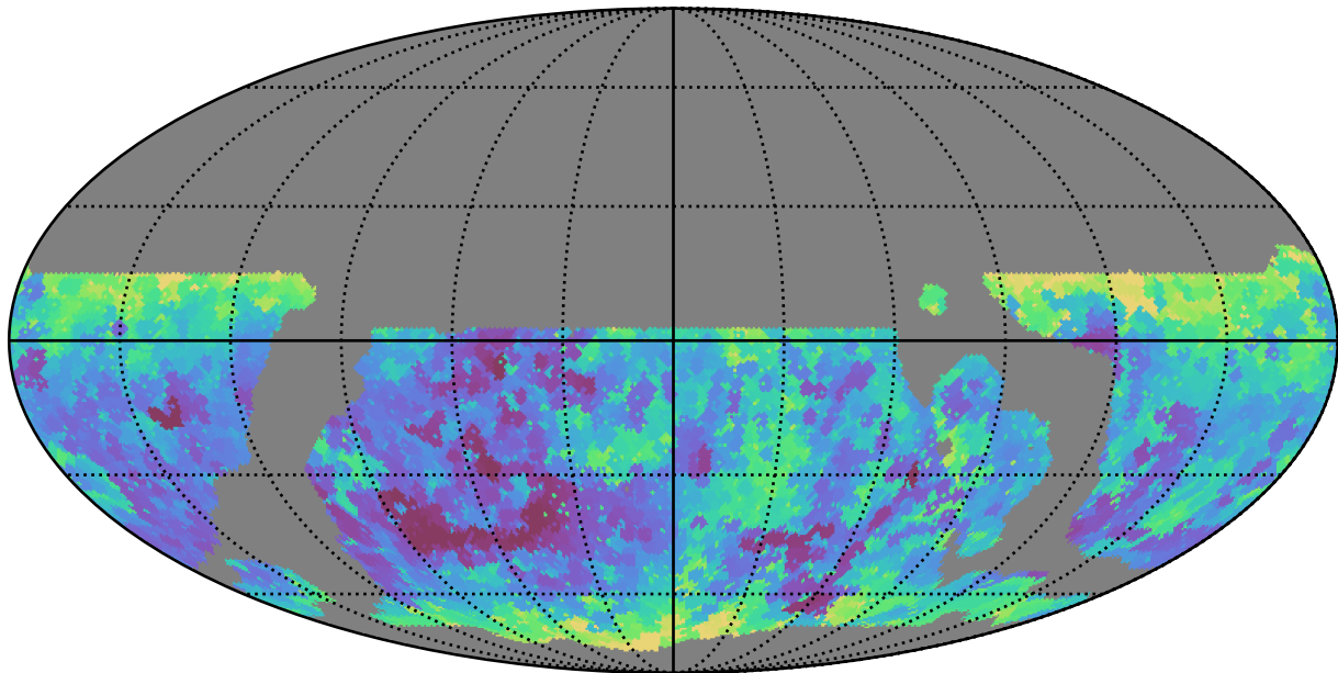
weather_cloudso10v3.4_10yrs WFD y band: Min seeingEff
