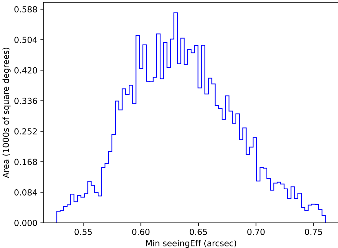
weather_cloudso10v3.4_10yrs WFD y band: Min seeingEff
