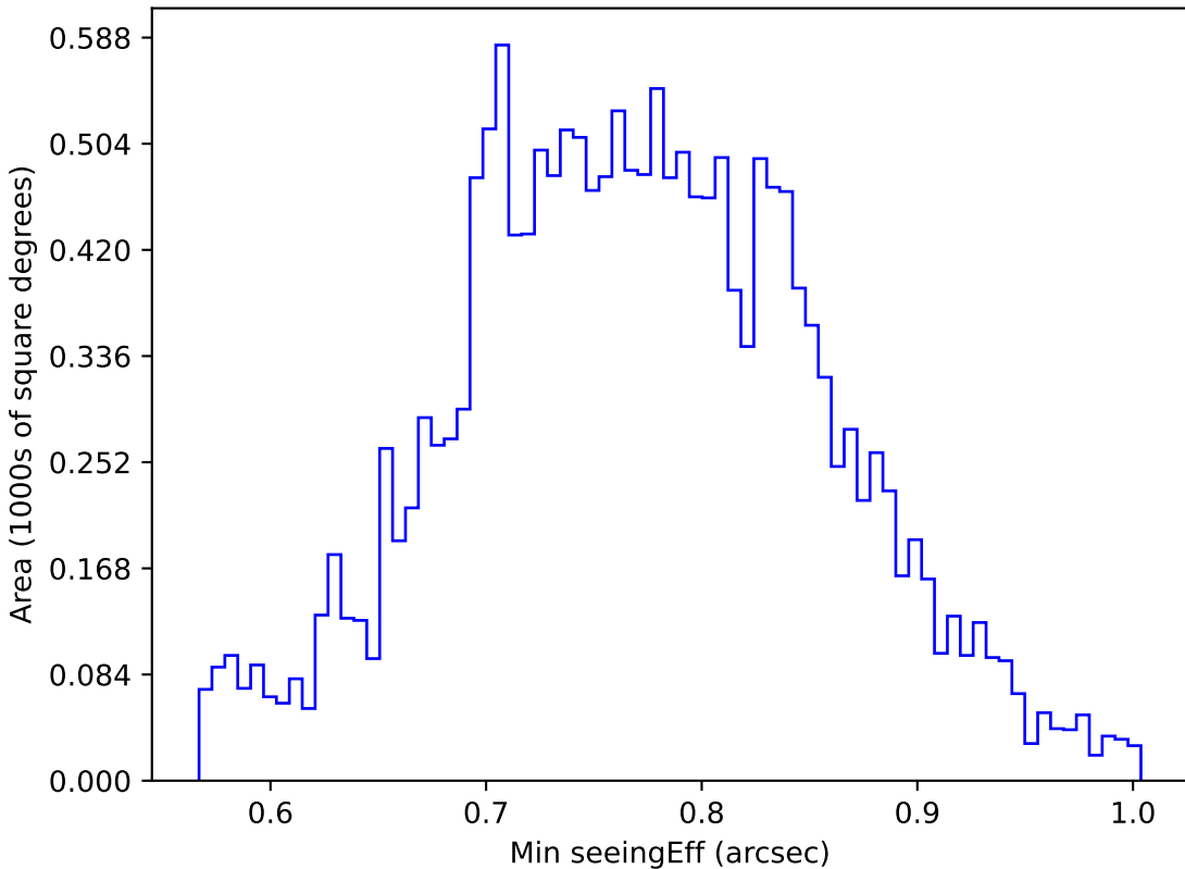
weather_cloudso10v3.4_10yrs WFD u band: Min seeingEff
