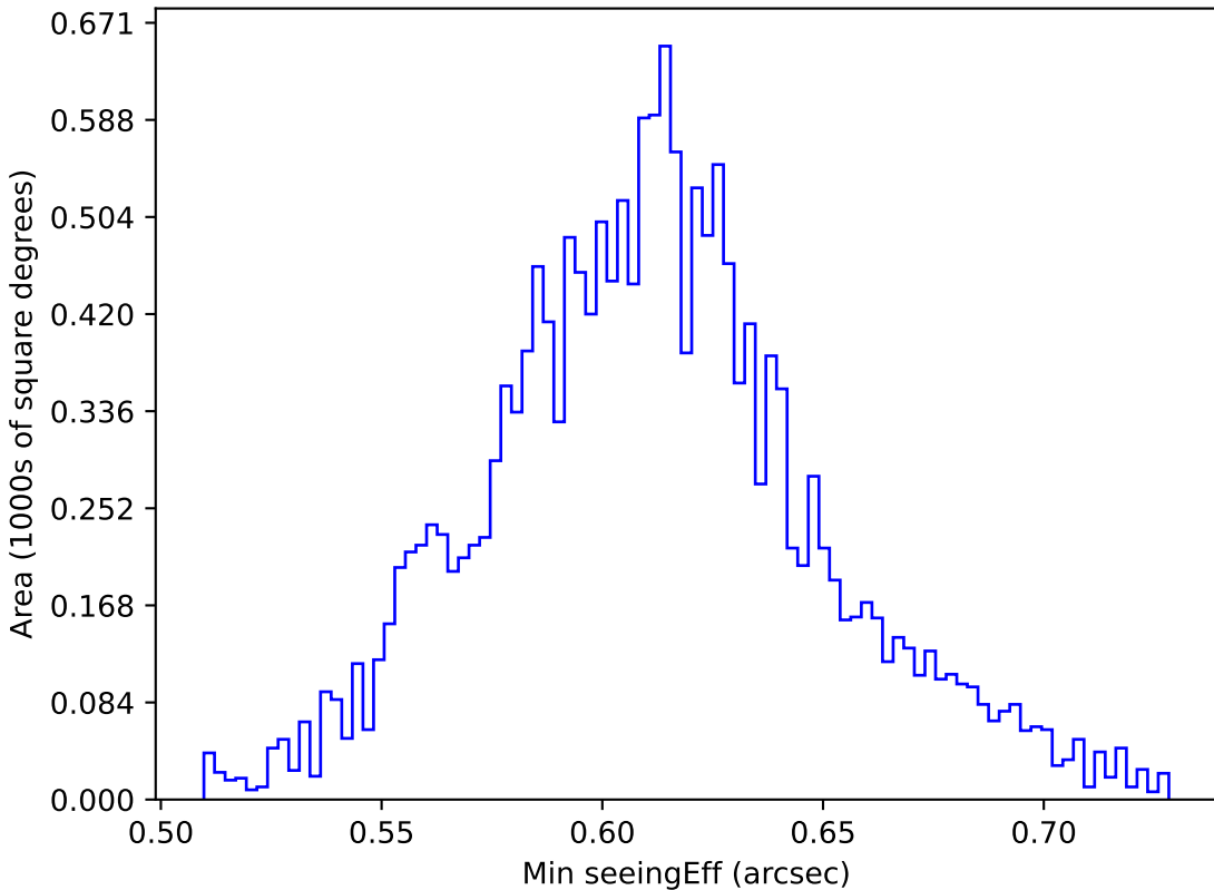
weather_cloudso10v3.4_10yrs WFD i band: Min seeingEff
