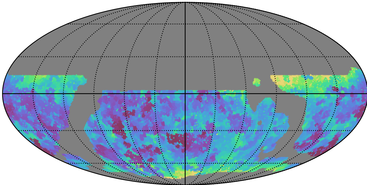
weather_cloudso10v3.4_10yrs WFD g band: Min seeingEff
