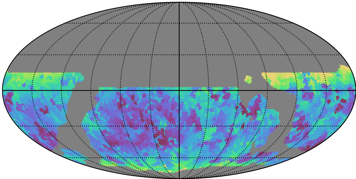
weather_cloudso10v3.4_10yrs WFD all bands: Min seeingEff
