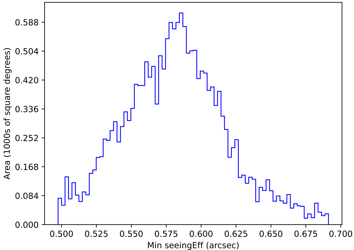
weather_cloudso10v3.4_10yrs WFD all bands: Min seeingEff
