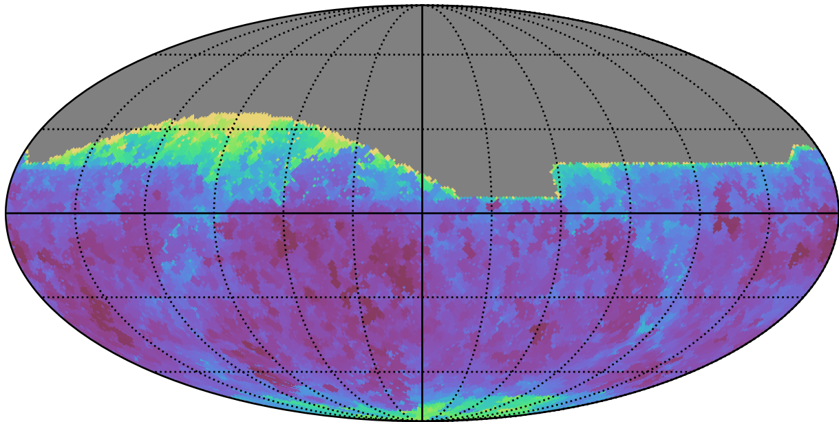
weather_cloudso10v3.4_10yrs All sky z band: Min seeingEff
