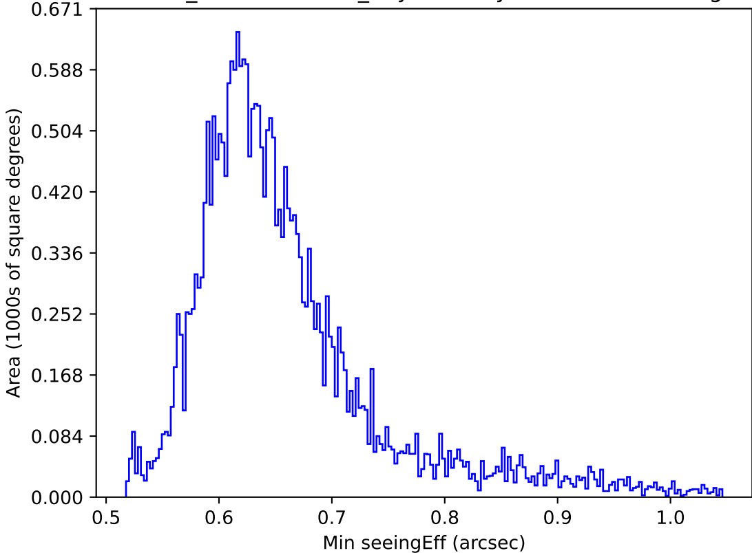
weather_cloudso10v3.4_10yrs All sky z band: Min seeingEff
