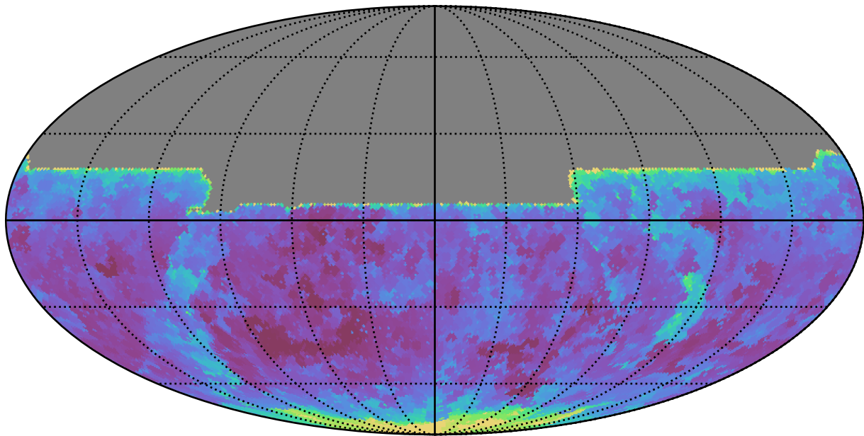
weather_cloudso10v3.4_10yrs All sky y band: Min seeingEff
