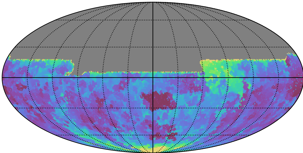
weather_cloudso10v3.4_10yrs All sky u band: Min seeingEff
