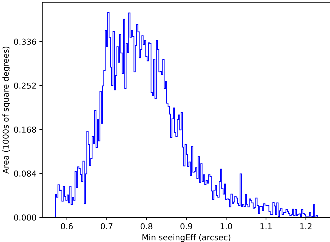
weather_cloudso10v3.4_10yrs All sky u band: Min seeingEff
