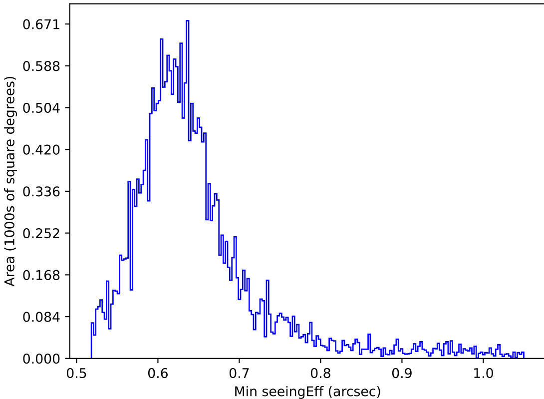
weather_cloudso10v3.4_10yrs All sky r band: Min seeingEff
