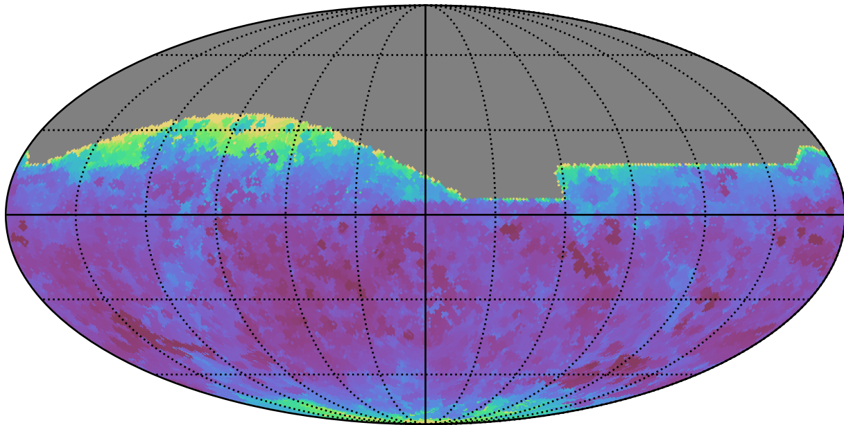
weather_cloudso10v3.4_10yrs All sky i band: Min seeingEff
