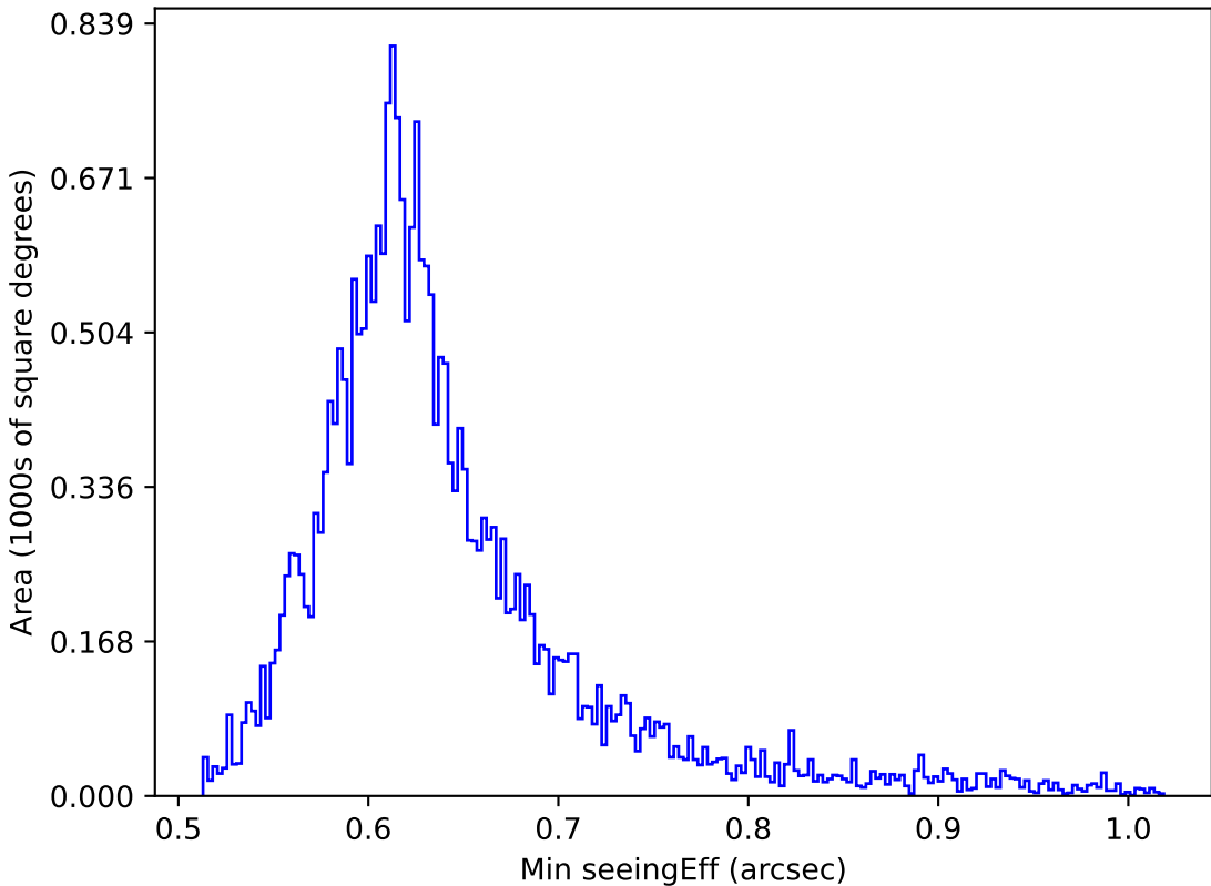
weather_cloudso10v3.4_10yrs All sky i band: Min seeingEff
