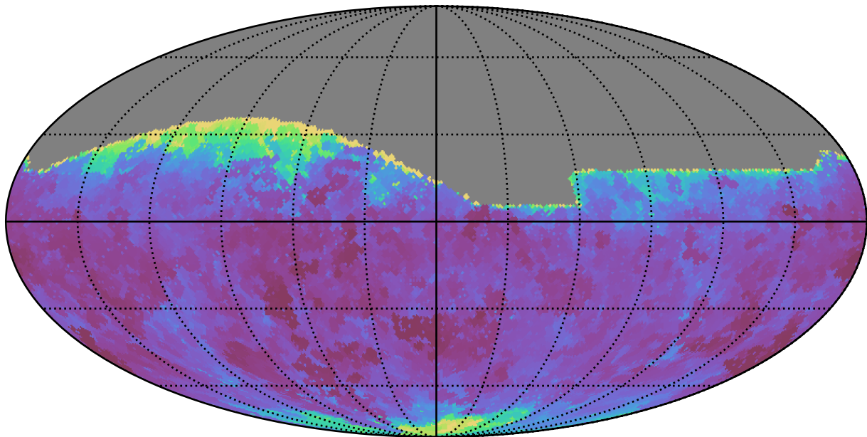
weather_cloudso10v3.4_10yrs All sky g band: Min seeingEff
