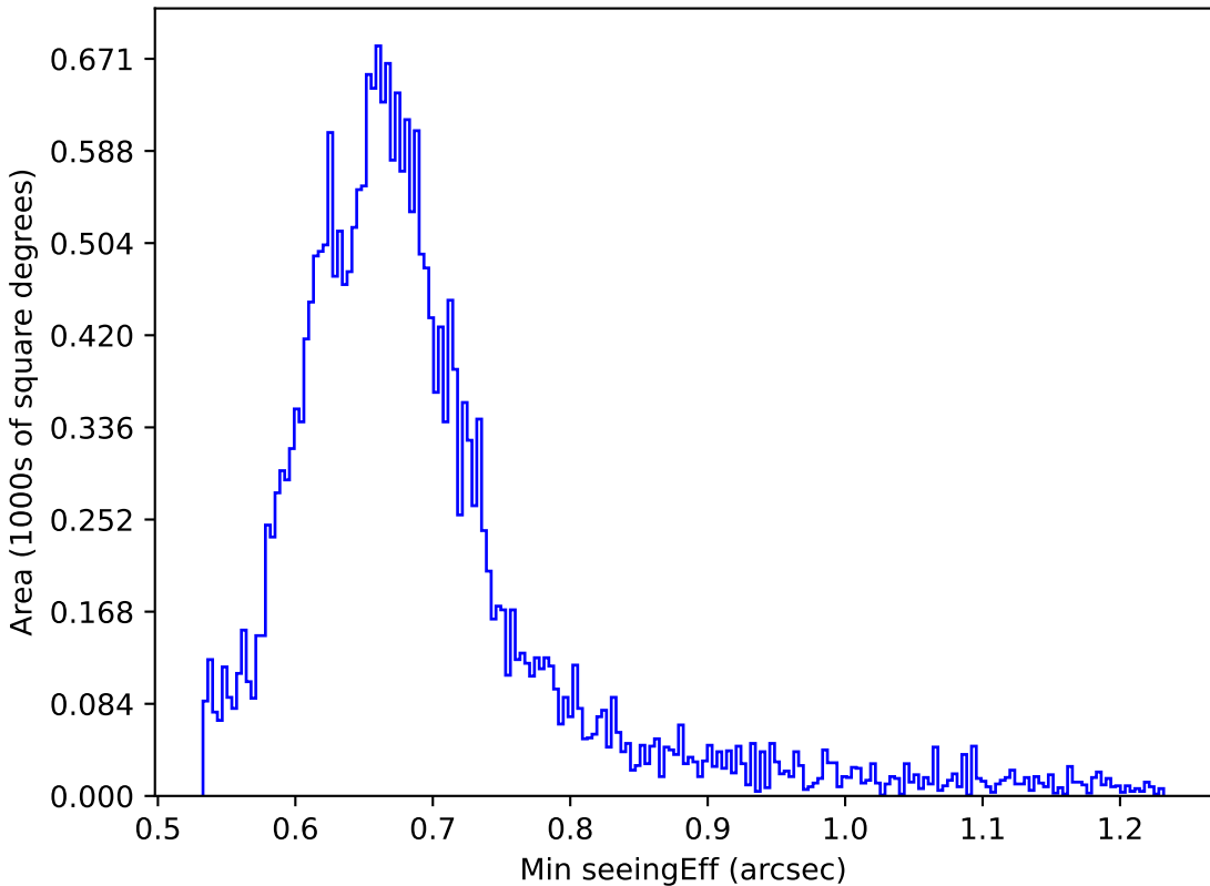
weather_cloudso10v3.4_10yrs All sky g band: Min seeingEff
