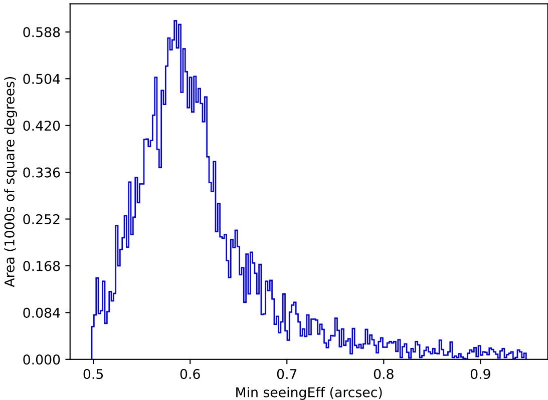
weather_cloudso10v3.4_10yrs All sky all bands: Min seeingEff
