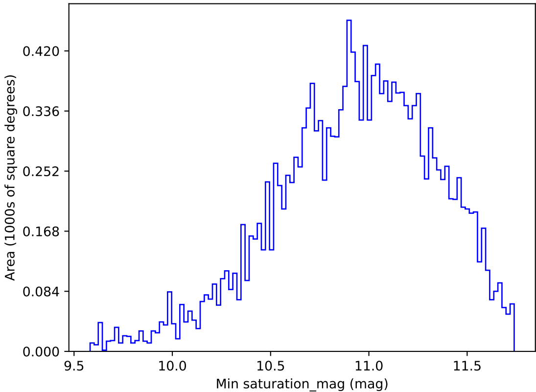
weather_cloudso10v3.4_10yrs WFD all bands: Min saturation_mag
