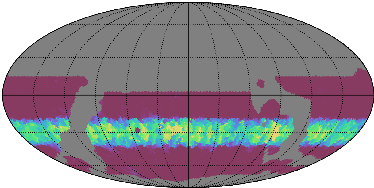
weather_cloudso10v3.4_10yrs WFD u band: Min normairmass
