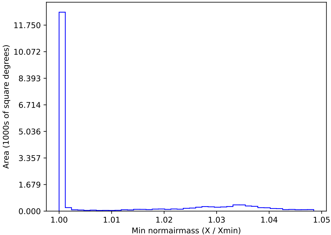
weather_cloudso10v3.4_10yrs WFD g band: Min normairmass
