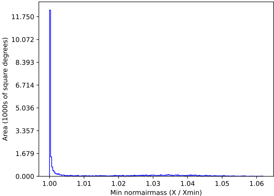
weather_cloudso10v3.4_10yrs All sky u band: Min normairmass
