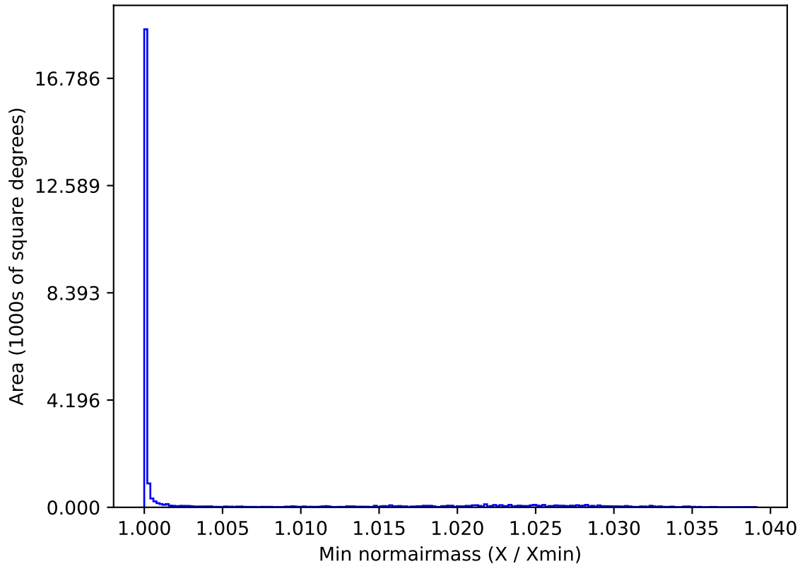
weather_cloudso10v3.4_10yrs All sky r band: Min normairmass
