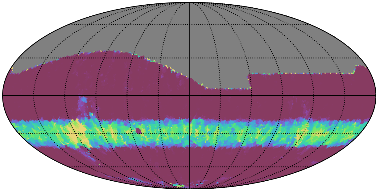
weather_cloudso10v3.4_10yrs All sky g band: Min normairmass
