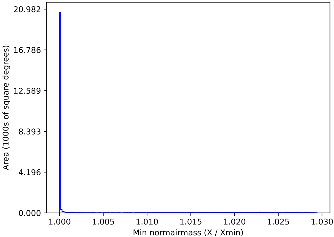
weather_cloudso10v3.4_10yrs All sky all bands: Min normairmass
