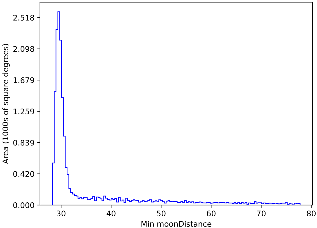
weather_cloudso10v3.4_10yrs WFD z band: Min moonDistance
