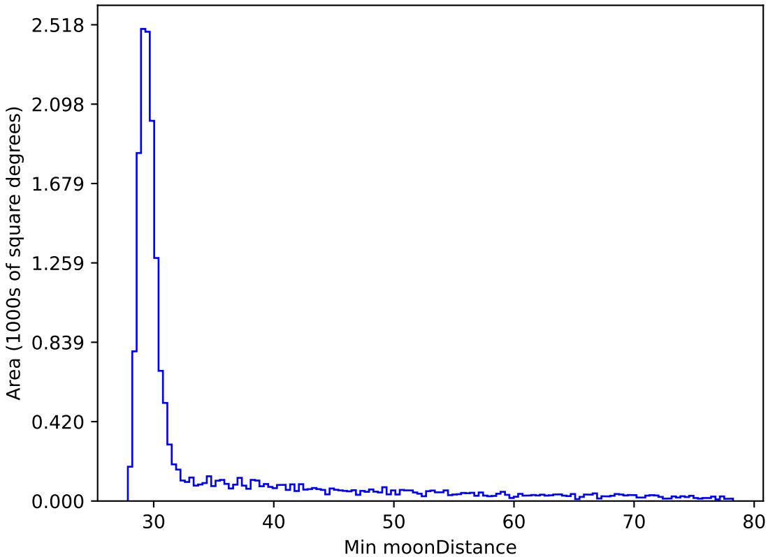
weather_cloudso10v3.4_10yrs WFD y band: Min moonDistance
