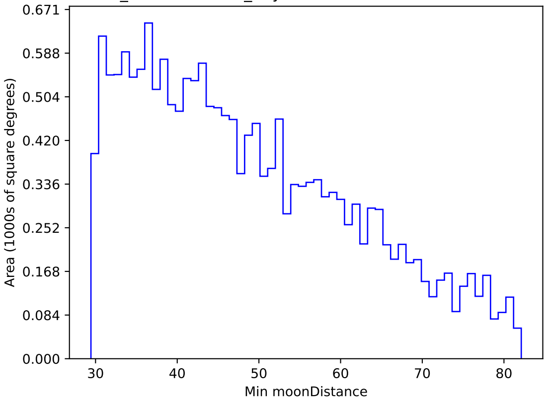
weather_cloudso10v3.4_10yrs WFD u band: Min moonDistance
