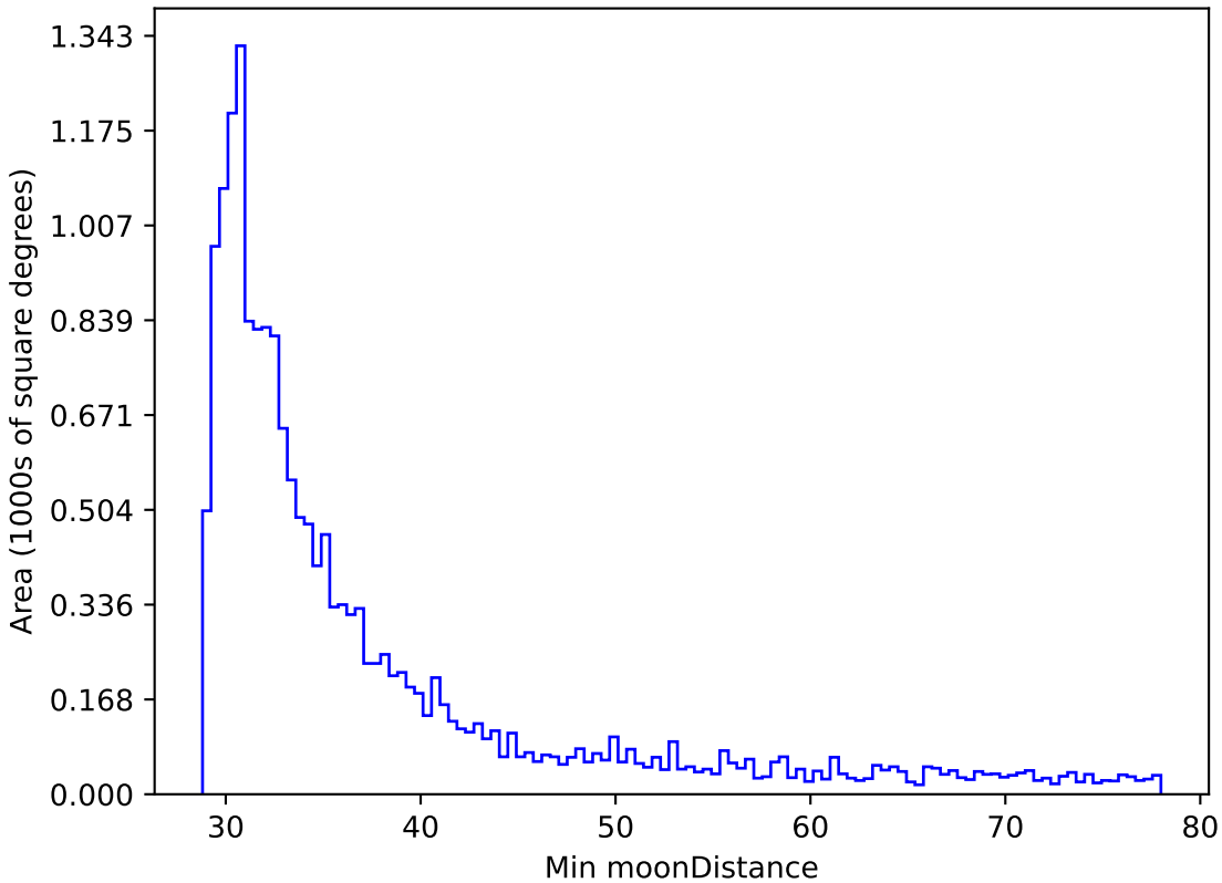
weather_cloudso10v3.4_10yrs WFD r band: Min moonDistance
