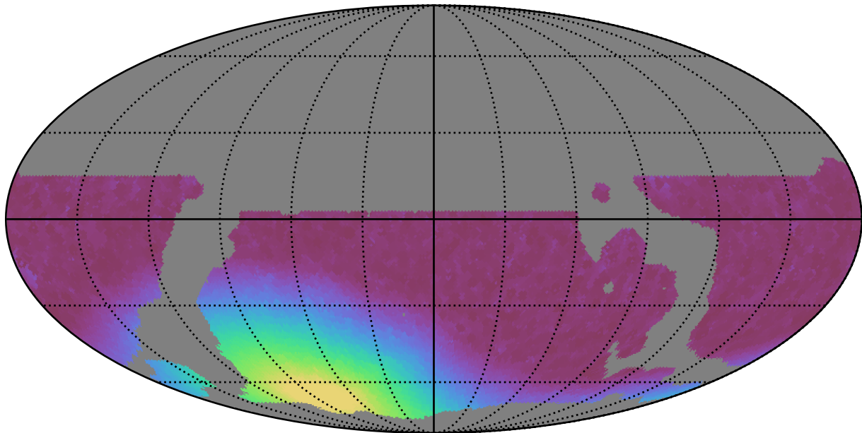
weather_cloudso10v3.4_10yrs WFD i band: Min moonDistance
