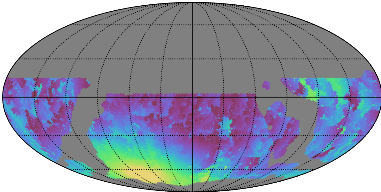
weather_cloudso10v3.4_10yrs WFD g band: Min moonDistance
