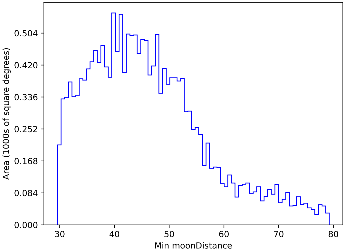
weather_cloudso10v3.4_10yrs WFD g band: Min moonDistance
